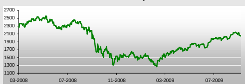
Nasdaq
